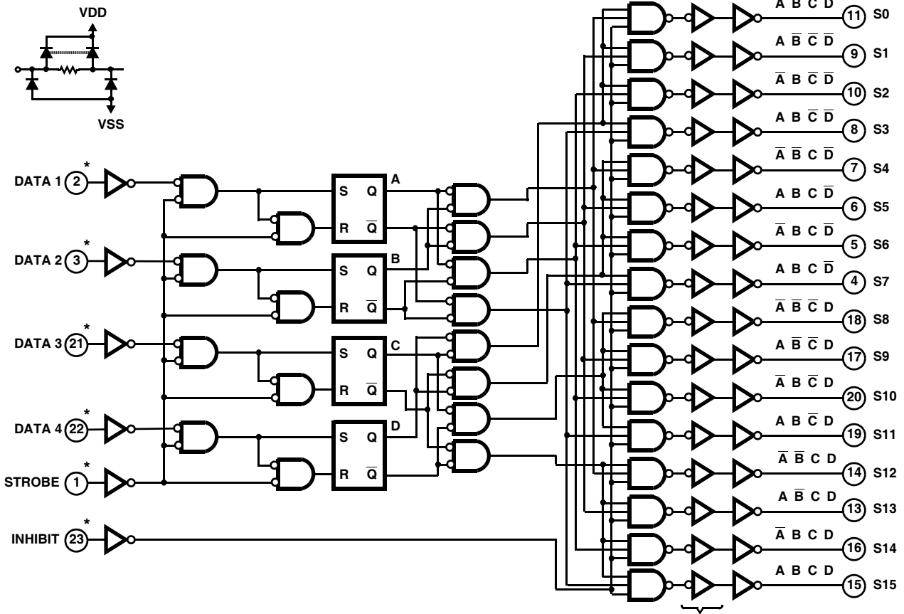
FIGURE 1. LOGIC DIAGRAM
