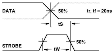
FIGURE 11. WAVEFORMS FOR SETUP TIME AND STROBE PULSE WIDTH
